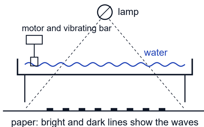
Ripple tank: measure \lambda and count waves on the paper below.
