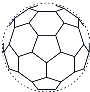
buckminsterfullerene, C 60
