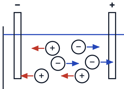
molten or dissolved: ions free to move, so it conducts
