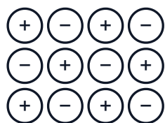
solid: ions fixed does not conduct
