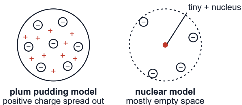
Plum pudding (left) and nuclear model (right).
