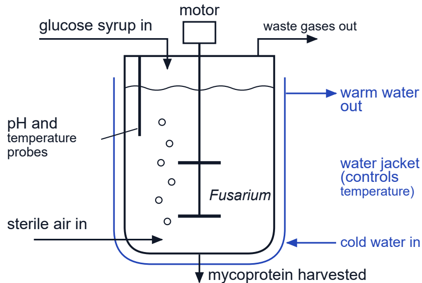
A fermenter for growing Fusarium
